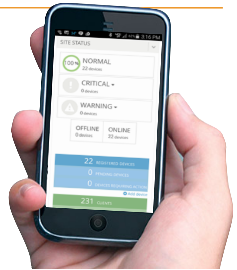
Responsive Layout
